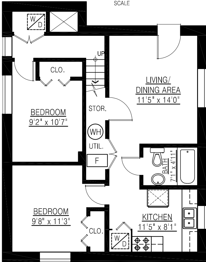
LOWER FLOOR PLAN FLOOR AREA: 840 sq.ft.
