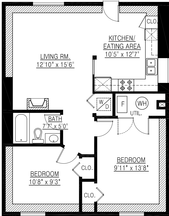
LOWER FLOOR PLAN FLOOR AREA: 917 sq.ft.
